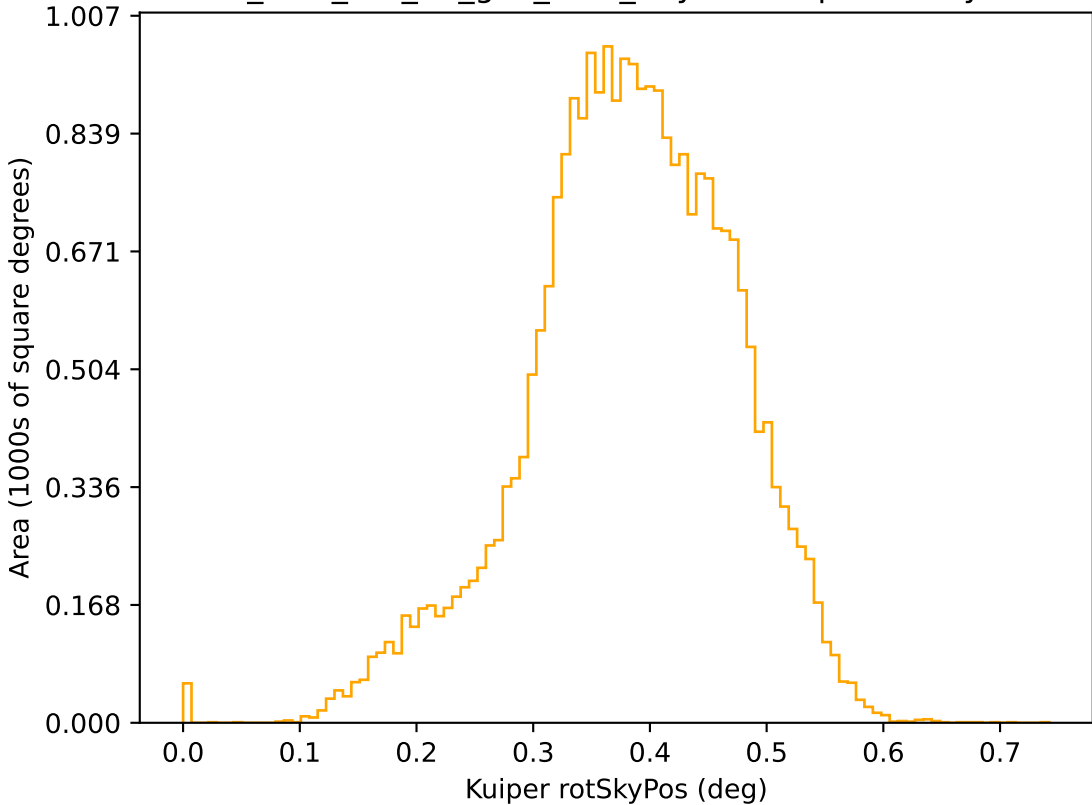
too_elab_r64_d3_griz_v3.4_10yrs r: Kuiper rotSkyPos
