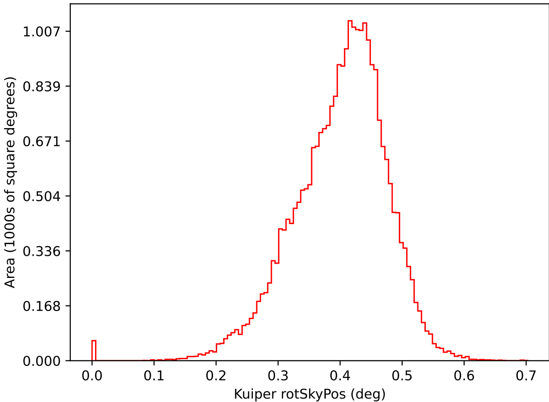
too_elab_r64_d3_griz_v3.4_10yrs i: Kuiper rotSkyPos
