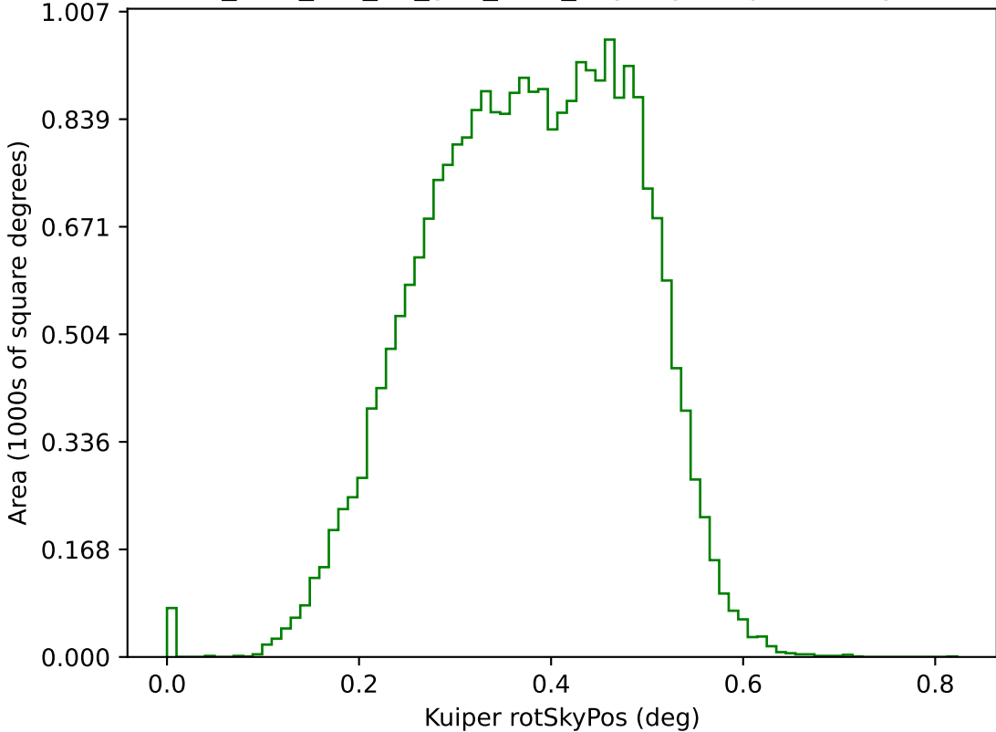
too_elab_r64_d3_griz_v3.4_10yrs g: Kuiper rotSkyPos
