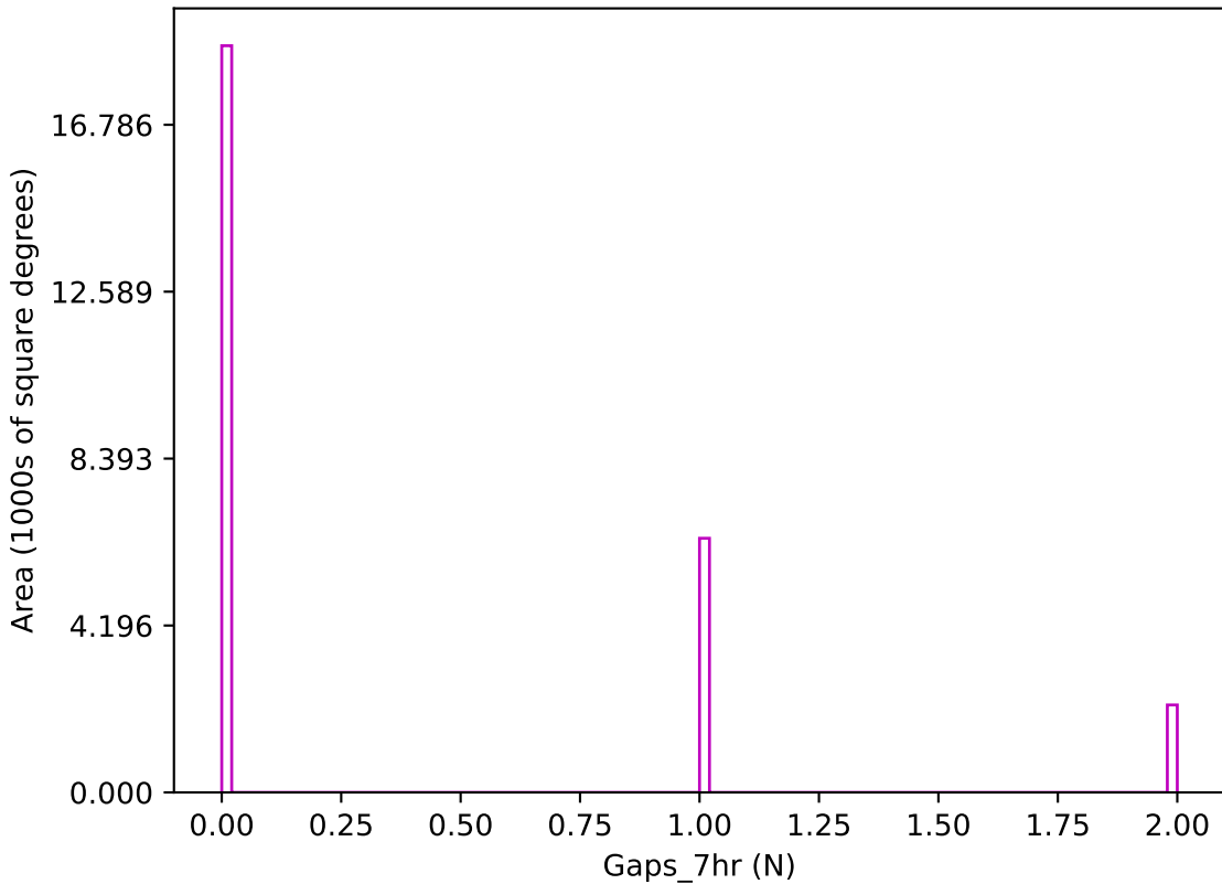
too_elab_r64_d3_griz_v3.4_10yrs z band: Gaps_7hr
