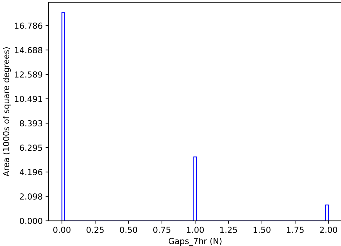
too_elab_r64_d3_griz_v3.4_10yrs y band: Gaps_7hr
