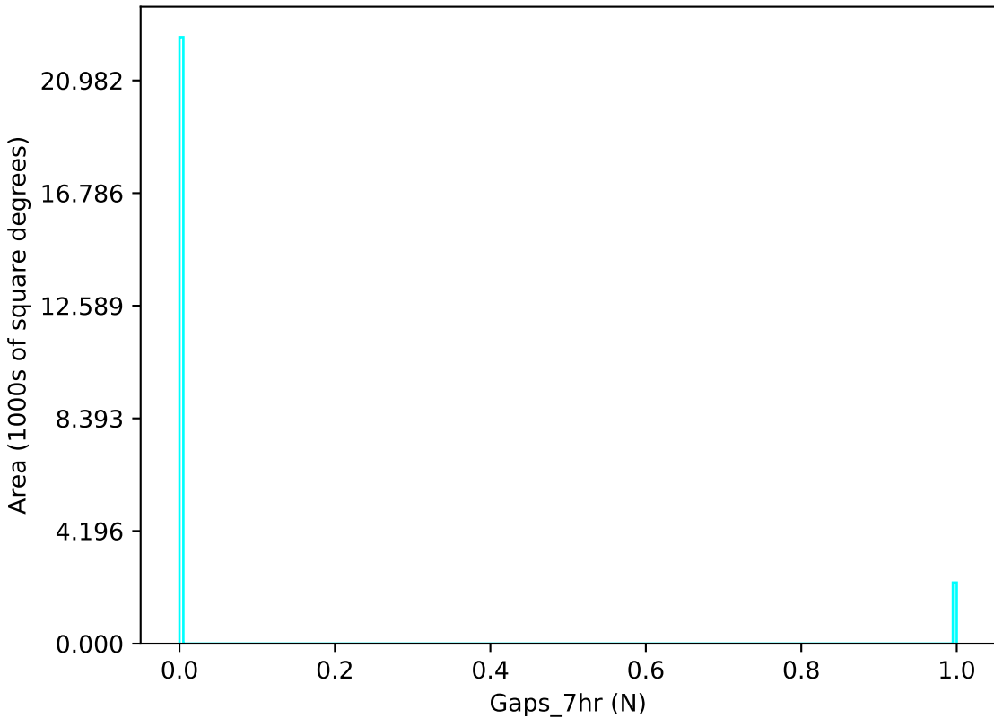
too_elab_r64_d3_griz_v3.4_10yrs u band: Gaps_7hr
