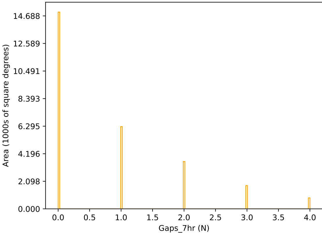
too_elab_r64_d3_griz_v3.4_10yrs r band: Gaps_7hr
