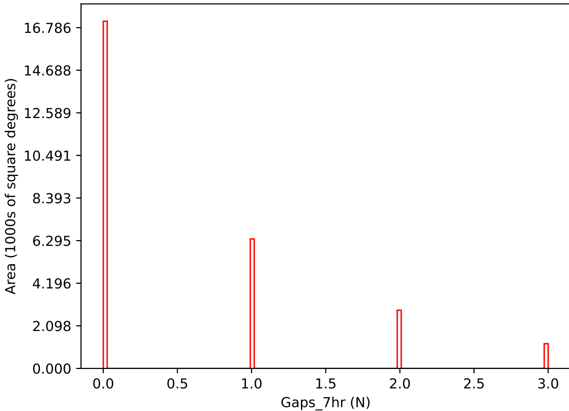
too_elab_r64_d3_griz_v3.4_10yrs i band: Gaps_7hr
