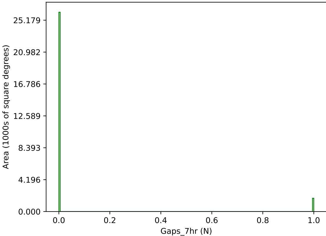
too_elab_r64_d3_griz_v3.4_10yrs g band: Gaps_7hr
