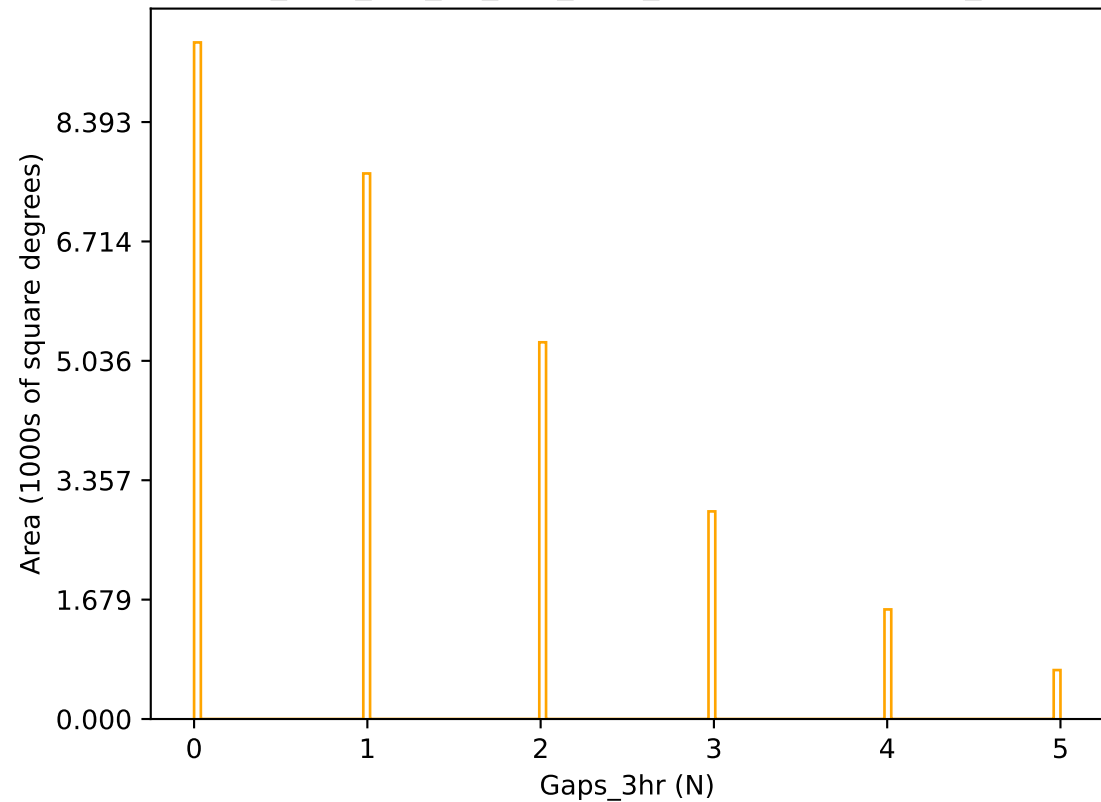
too_elab_r64_d3_griz_v3.4_10yrs r band: Gaps_3hr
