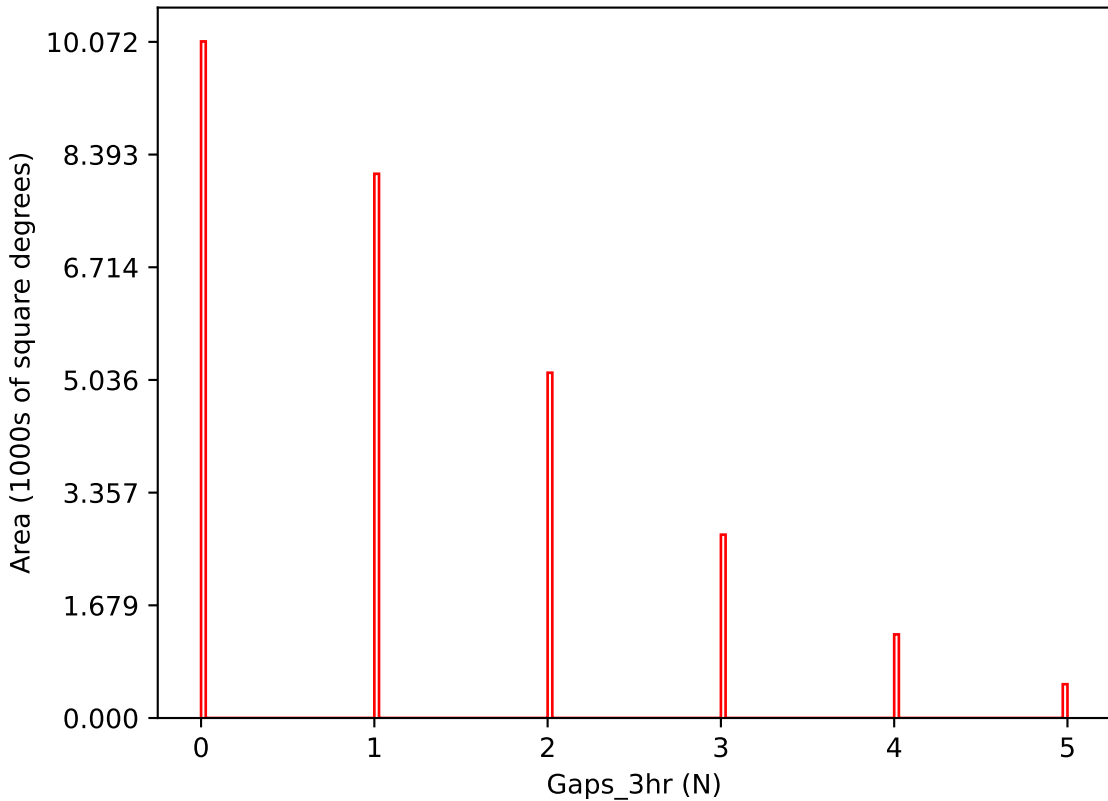
too_elab_r64_d3_griz_v3.4_10yrs i band: Gaps_3hr
