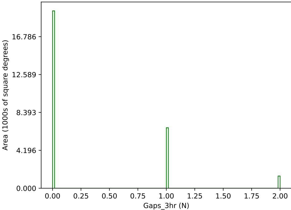
too_elab_r64_d3_griz_v3.4_10yrs g band: Gaps_3hr
