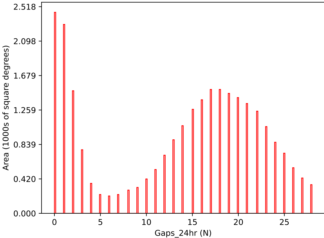
too_elab_r64_d3_griz_v3.4_10yrs i band: Gaps_24hr
