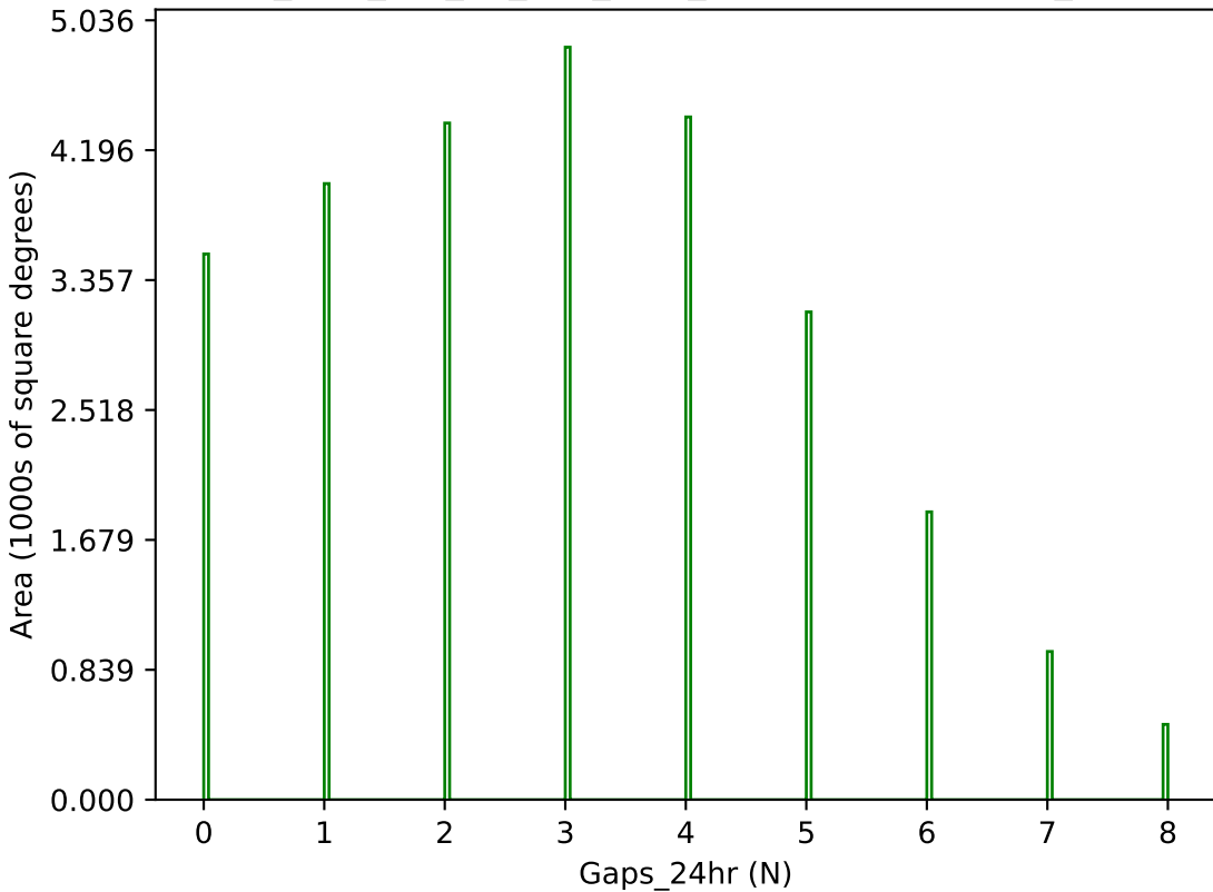
too_elab_r64_d3_griz_v3.4_10yrs g band: Gaps_24hr
