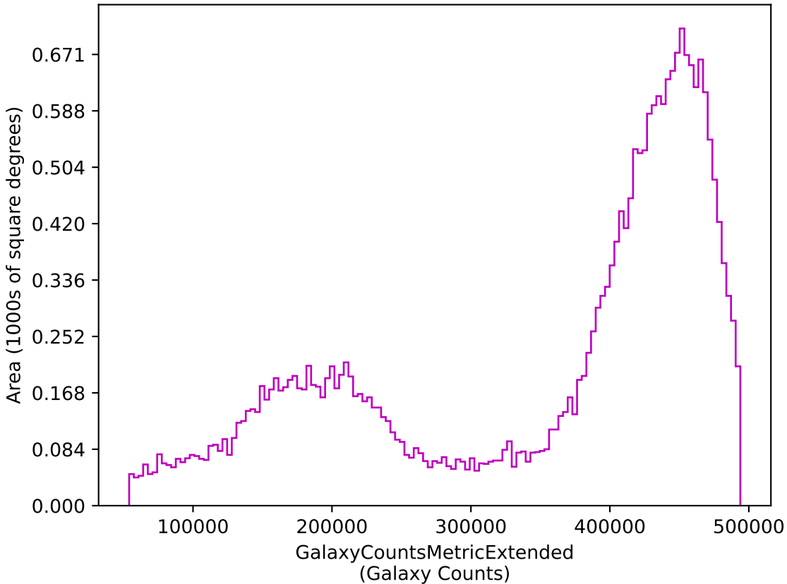
too_elab_r64_d3_griz_v3.4_10yrs z: GalaxyCountsMetricExtended
