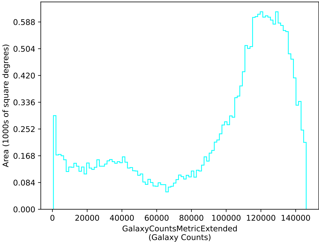
too_elab_r64_d3_griz_v3.4_10yrs u: GalaxyCountsMetricExtended
