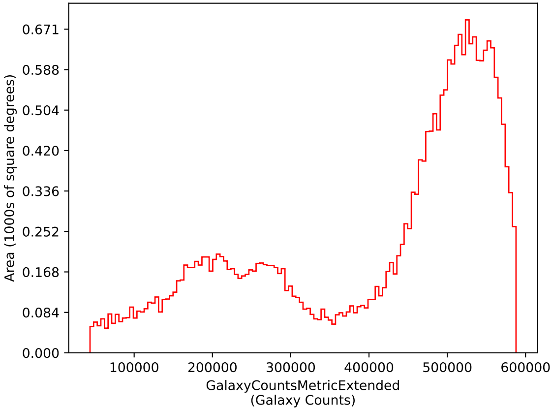
too_elab_r64_d3_griz_v3.4_10yrs i: GalaxyCountsMetricExtended
