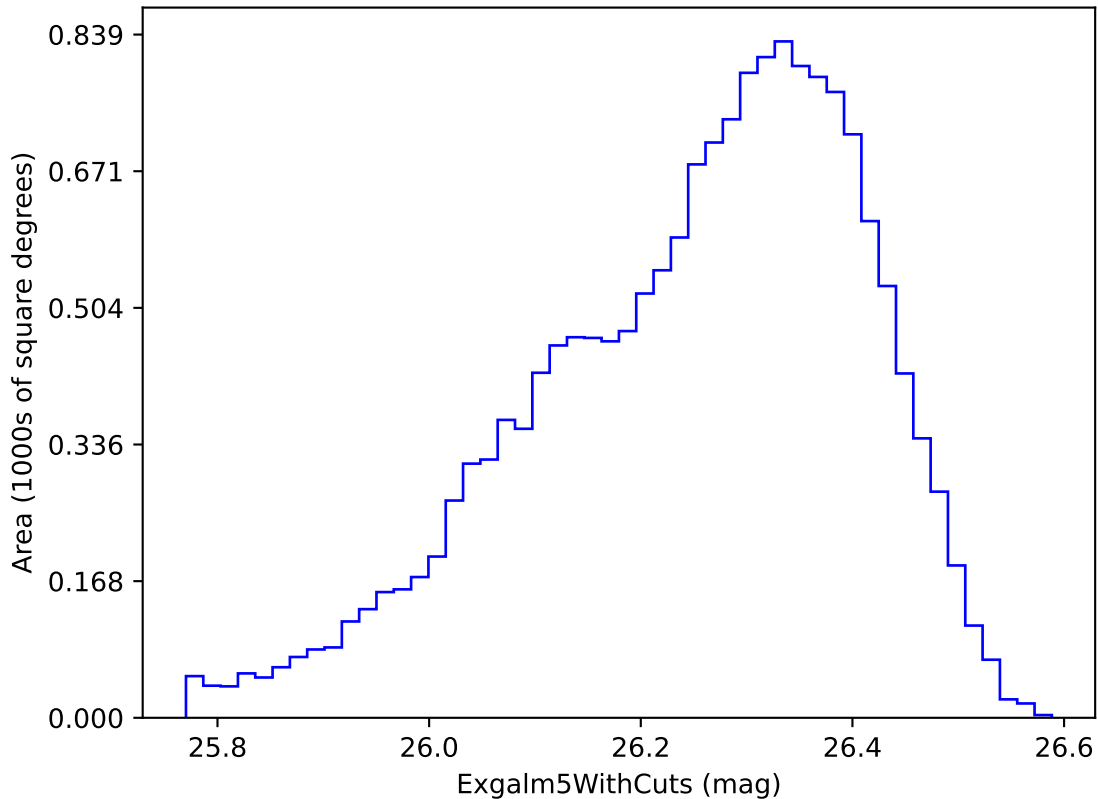
too_elab_r64_d3_griz_v3.4_10yrs i band non-DD year 8: ExgalM5WithCuts
