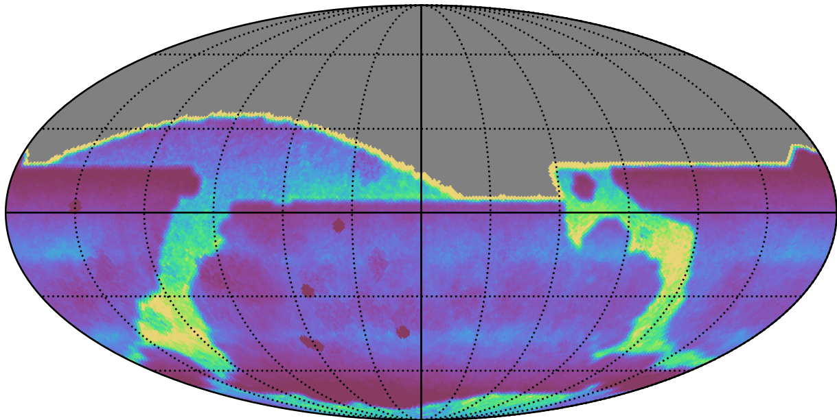
too_elab_r64_d3_griz_v3.4_10yrs : DCRprecision
