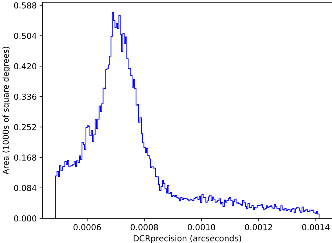
too_elab_r64_d3_griz_v3.4_10yrs : DCRprecision
