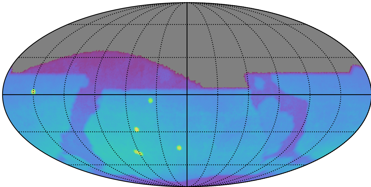
too_elab_r64_d3_griz_v3.4_10yrs : Brown Dwarf, L7
