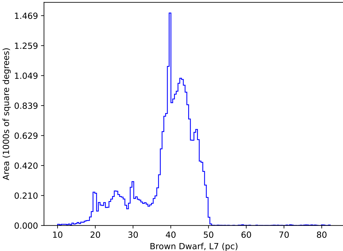
too_elab_r64_d3_griz_v3.4_10yrs : Brown Dwarf, L7
