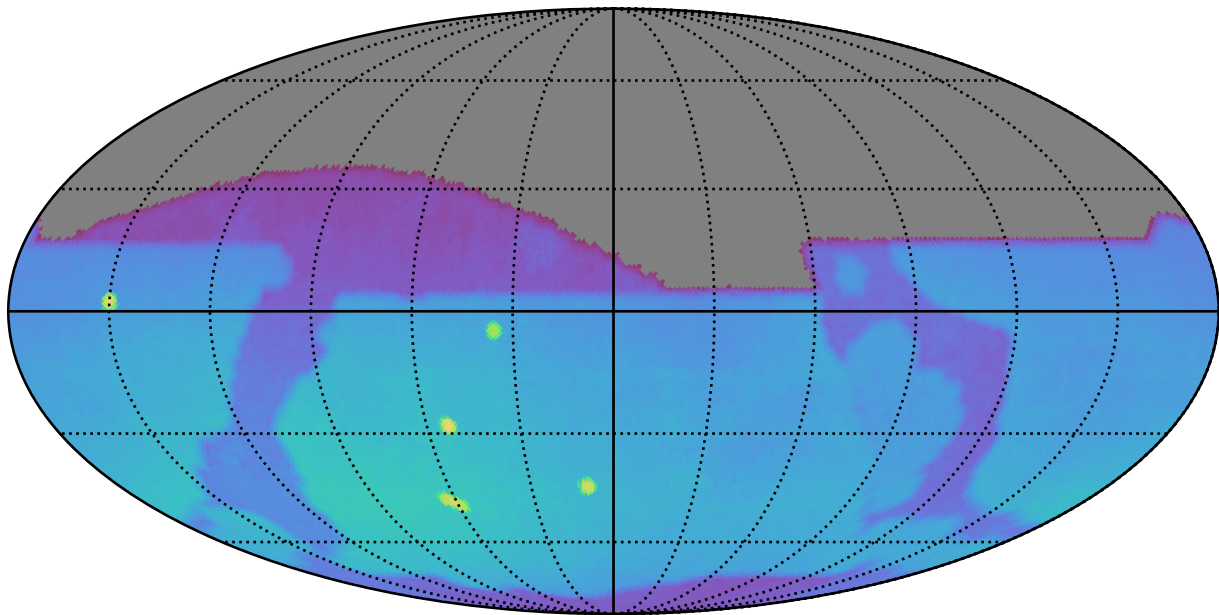
too_elab_r64_d3_griz_v3.4_10yrs : Brown Dwarf, L4
