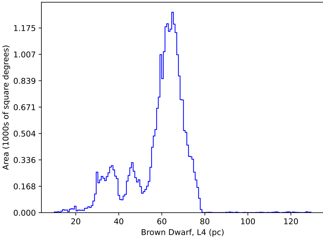
too_elab_r64_d3_griz_v3.4_10yrs : Brown Dwarf, L4
