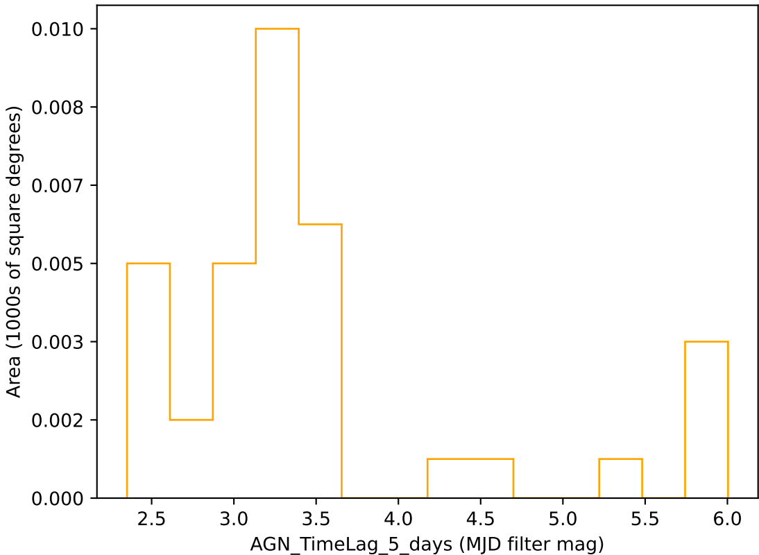
too_elab_r64_d3_griz_v3.4_10yrs r band: AGN_TimeLag_5_days
