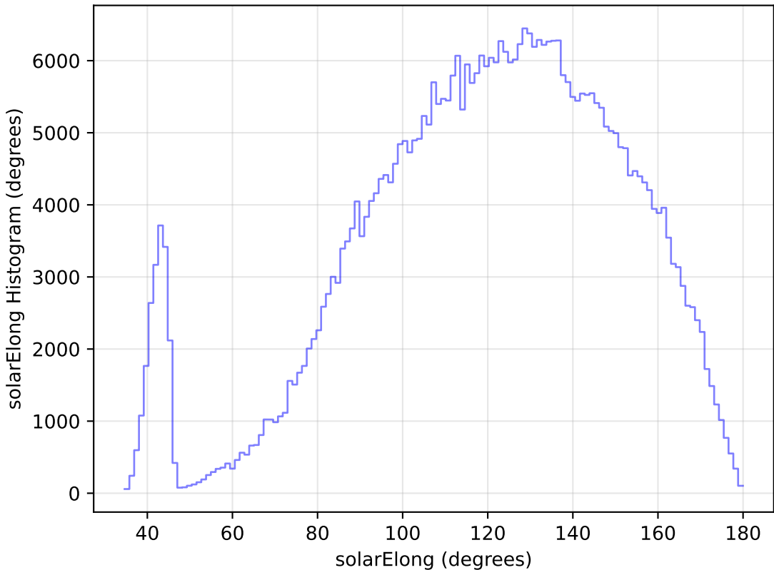
too_elab_r64_d3_griz_v3.4_10yrs WFD z band: solarElong Histogram
