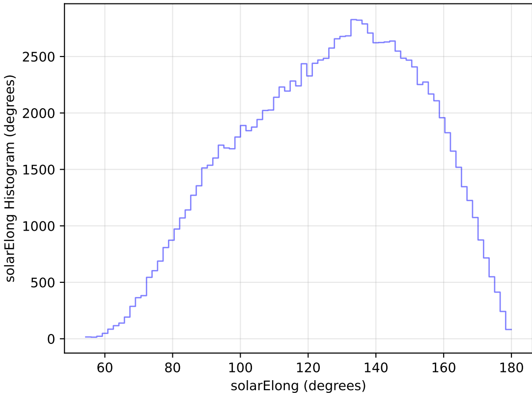
too_elab_r64_d3_griz_v3.4_10yrs WFD u band: solarElong Histogram
