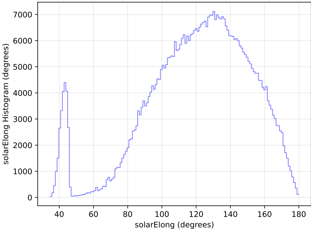
too_elab_r64_d3_griz_v3.4_10yrs WFD i band: solarElong Histogram
