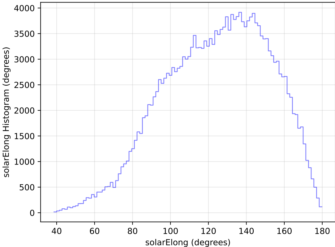
too_elab_r64_d3_griz_v3.4_10yrs WFD g band: solarElong Histogram
