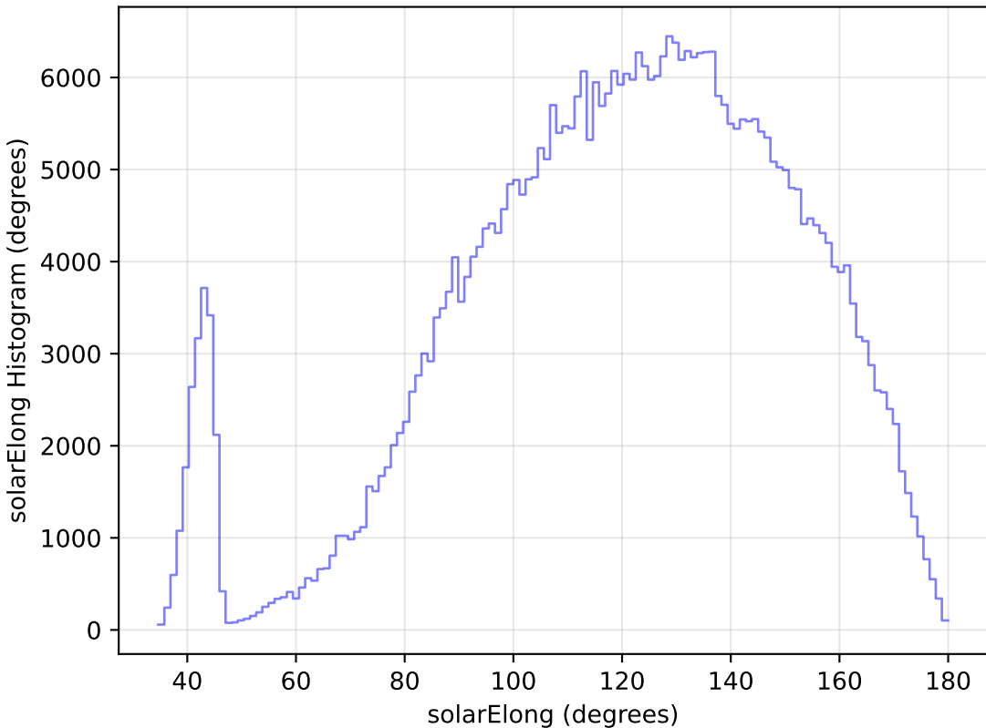
too_elab_r64_d3_griz_v3.4_10yrs All sky z band: solarElong Histogram
