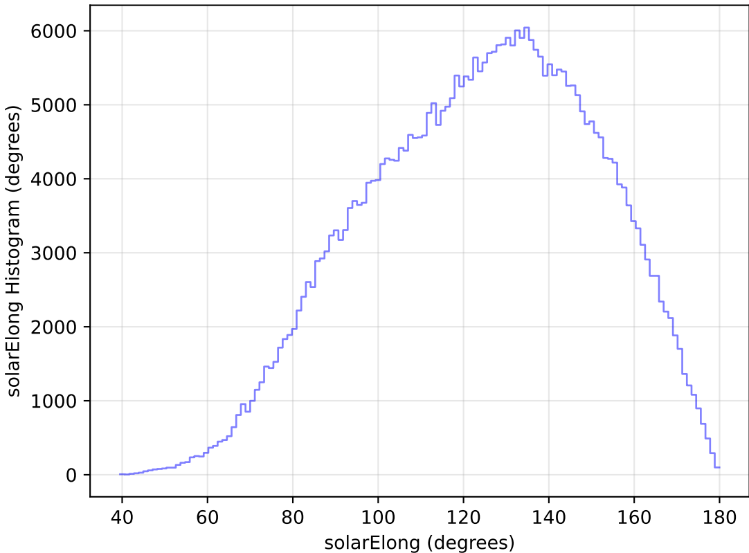
too_elab_r64_d3_griz_v3.4_10yrs All sky y band: solarElong Histogram
