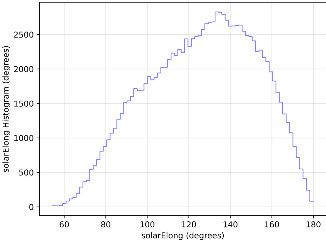
too_elab_r64_d3_griz_v3.4_10yrs All sky u band: solarElong Histogram
