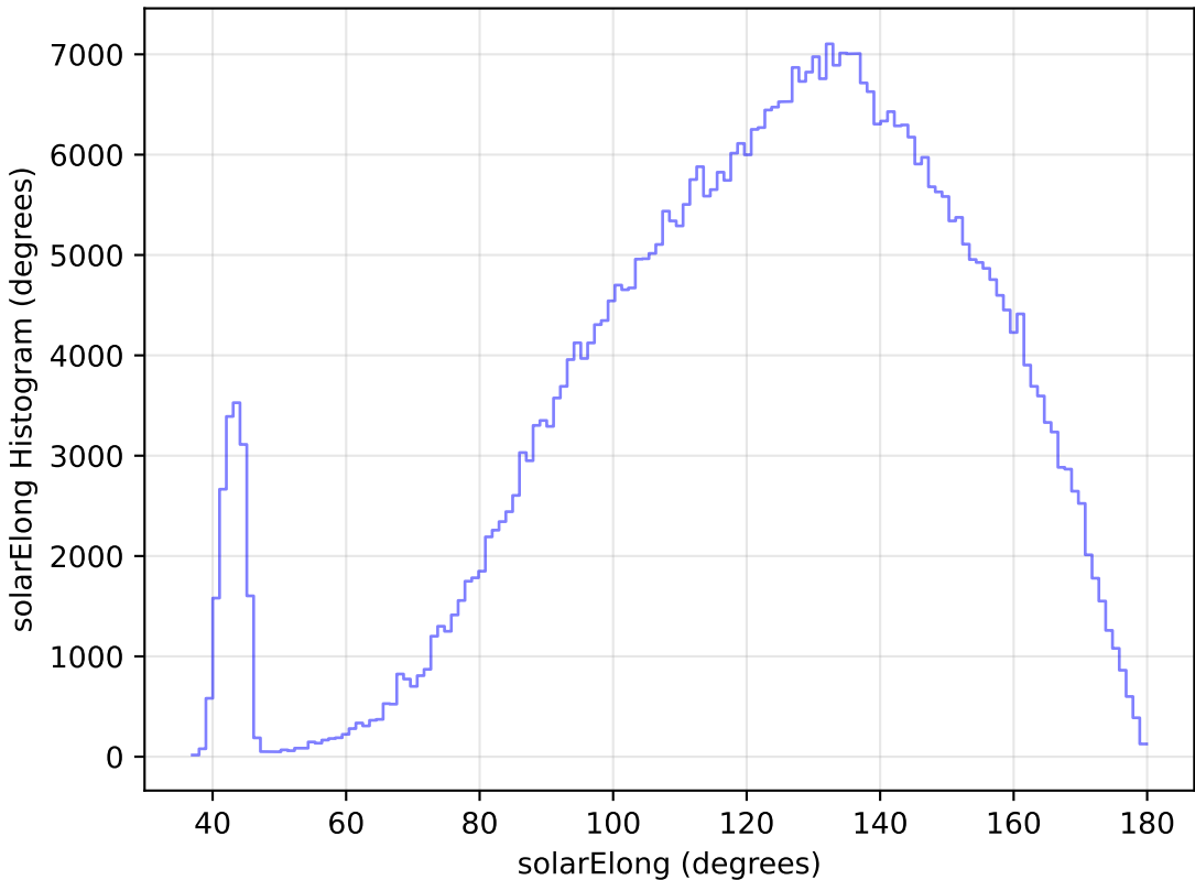
too_elab_r64_d3_griz_v3.4_10yrs All sky r band: solarElong Histogram
