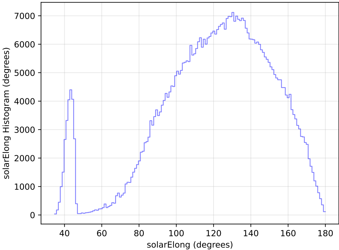
too_elab_r64_d3_griz_v3.4_10yrs All sky i band: solarElong Histogram
