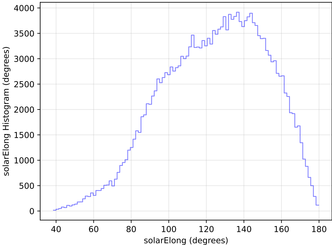
too_elab_r64_d3_griz_v3.4_10yrs All sky g band: solarElong Histogram
