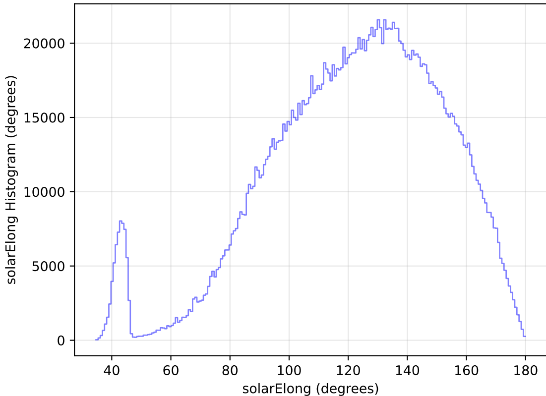
too_elab_r64_d3_griz_v3.4_10yrs All sky all bands: solarElong Histogram
