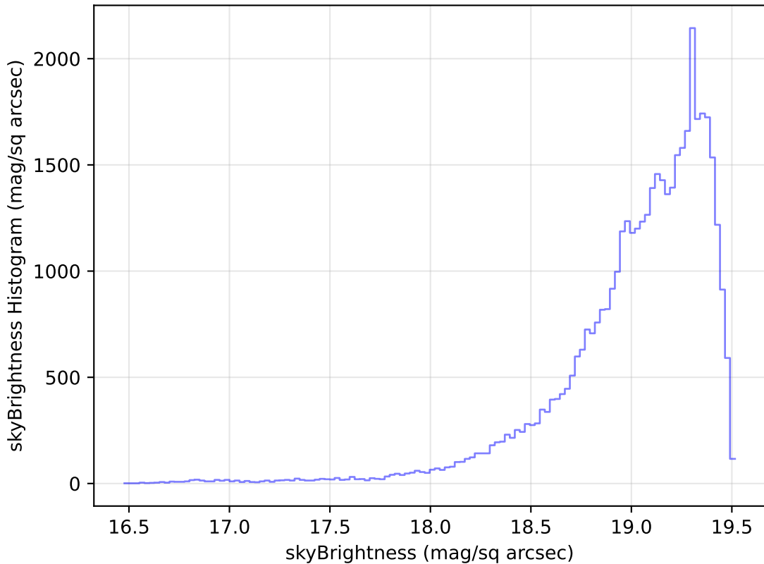
too_elab_r64_d3_griz_v3.4_10yrs Yr 1 z band: skyBrightness Histogram
