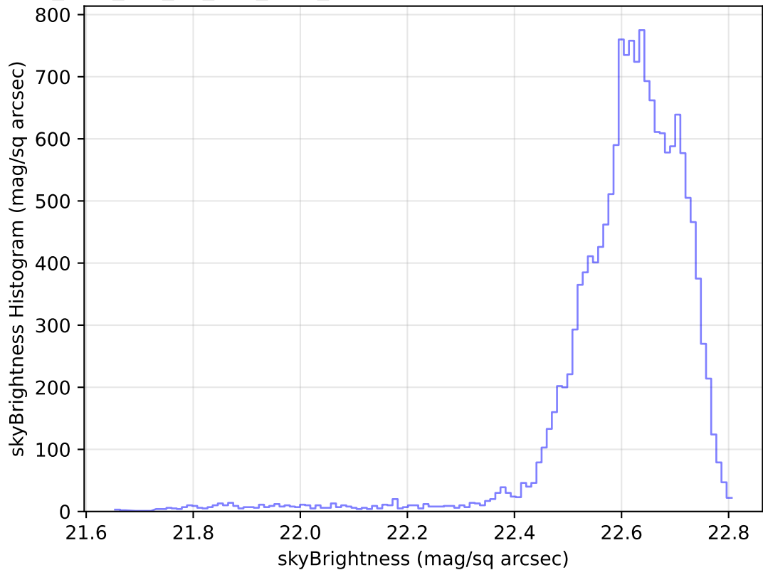
too_elab_r64_d3_griz_v3.4_10yrs Yr 1 u band: skyBrightness Histogram
