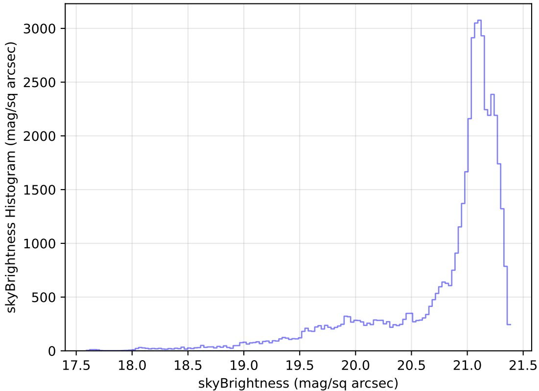
too_elab_r64_d3_griz_v3.4_10yrs Yr 1 r band: skyBrightness Histogram
