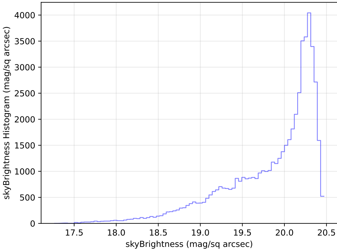
too_elab_r64_d3_griz_v3.4_10yrs Yr 1 i band: skyBrightness Histogram
