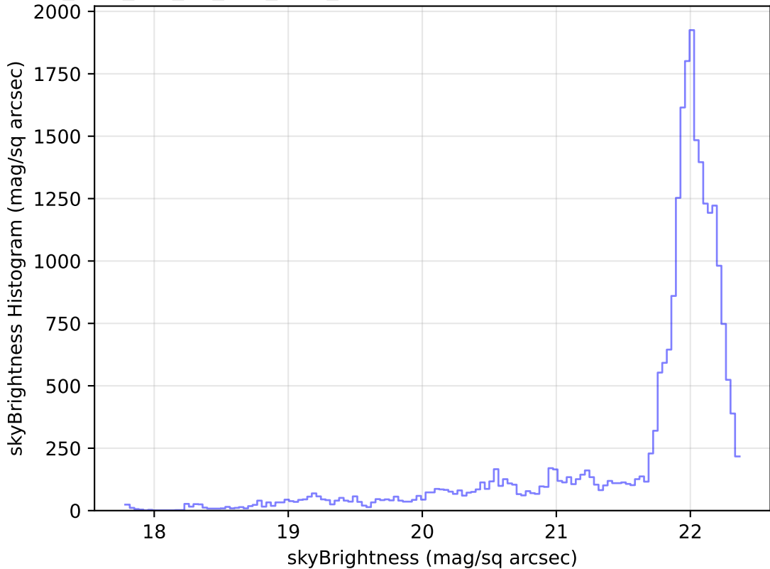
too_elab_r64_d3_griz_v3.4_10yrs Yr 1 g band: skyBrightness Histogram
