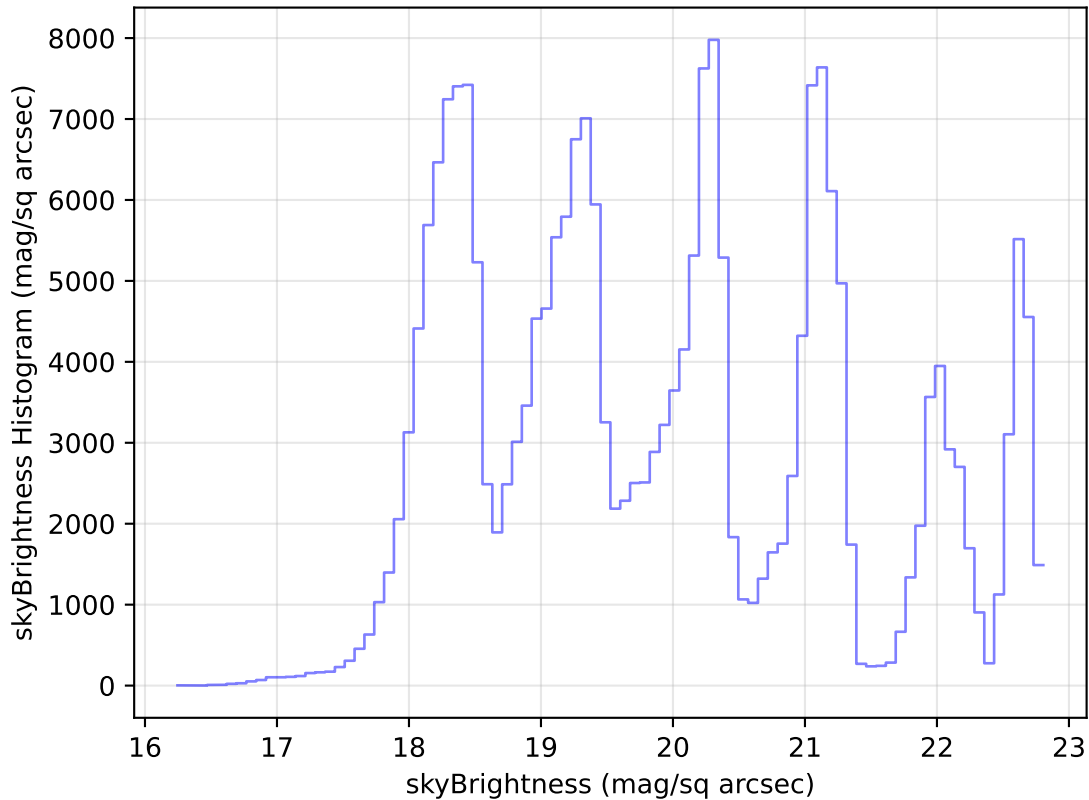
too_elab_r64_d3_griz_v3.4_10yrs Yr 1 all bands: skyBrightness Histogram
