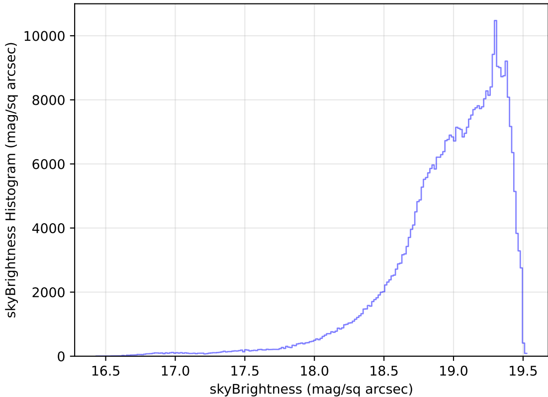
too_elab_r64_d3_griz_v3.4_10yrs WFD z band: skyBrightness Histogram
