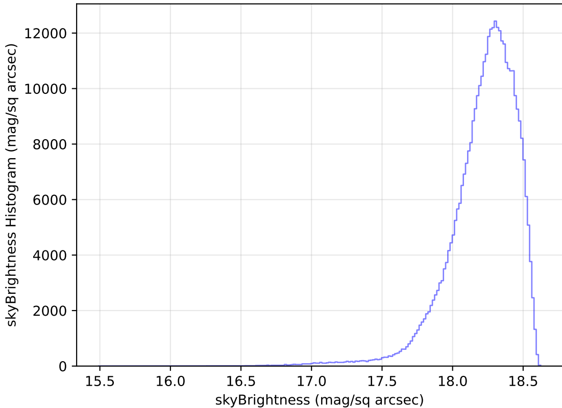
too_elab_r64_d3_griz_v3.4_10yrs WFD y band: skyBrightness Histogram
