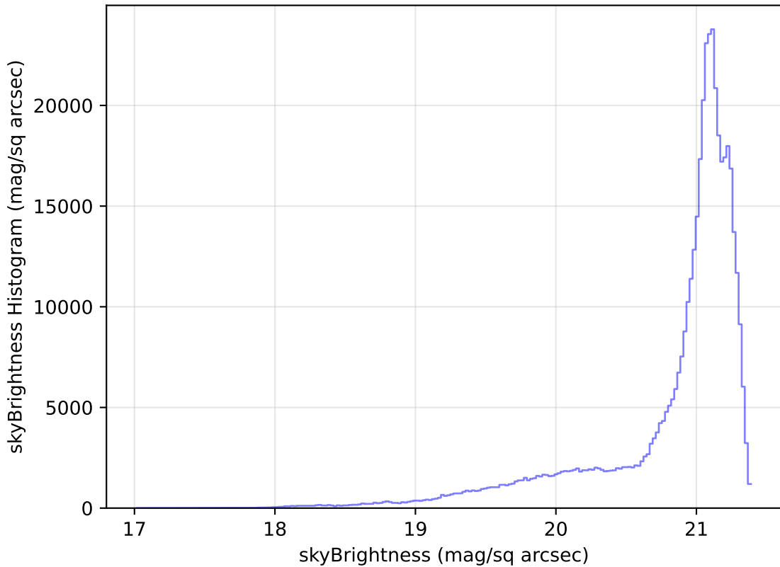
too_elab_r64_d3_griz_v3.4_10yrs WFD r band: skyBrightness Histogram
