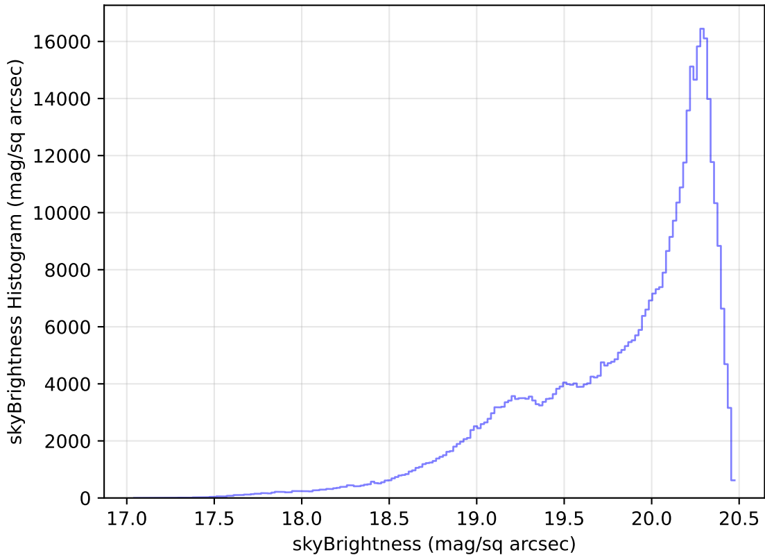
too_elab_r64_d3_griz_v3.4_10yrs WFD i band: skyBrightness Histogram
