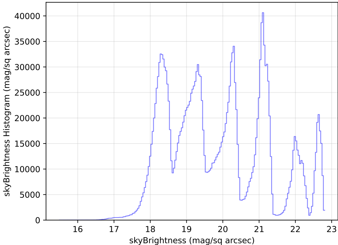
too_elab_r64_d3_griz_v3.4_10yrs WFD all bands: skyBrightness Histogram
