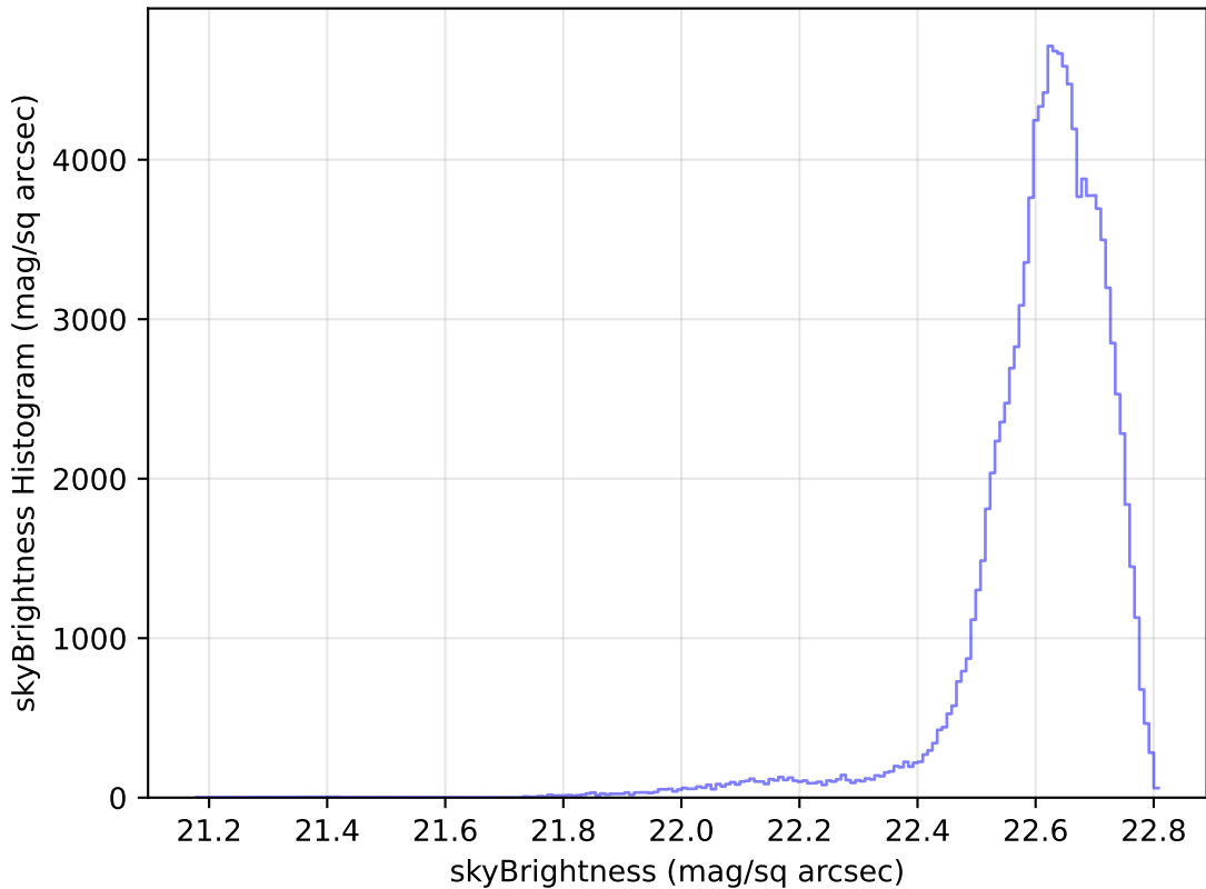
too_elab_r64_d3_griz_v3.4_10yrs All sky u band: skyBrightness Histogram
