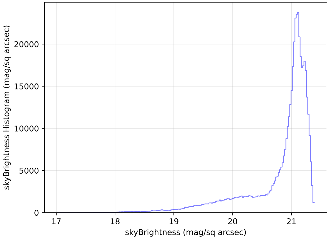
too_elab_r64_d3_griz_v3.4_10yrs All sky r band: skyBrightness Histogram
