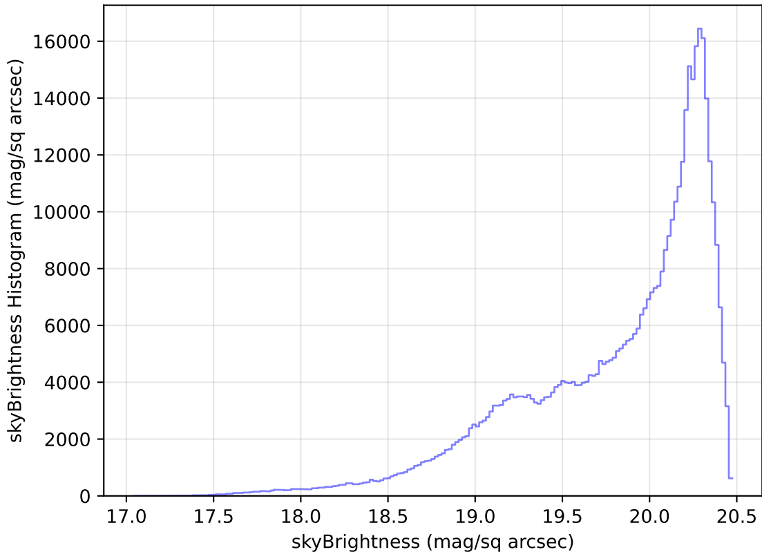
too_elab_r64_d3_griz_v3.4_10yrs All sky i band: skyBrightness Histogram
